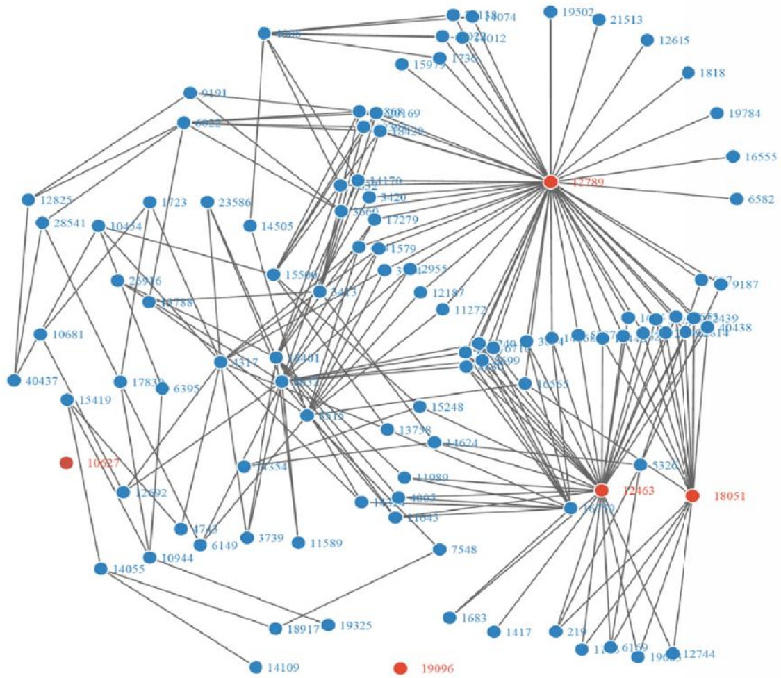
Figure 4 – Network of Lambda Matrix 2013
