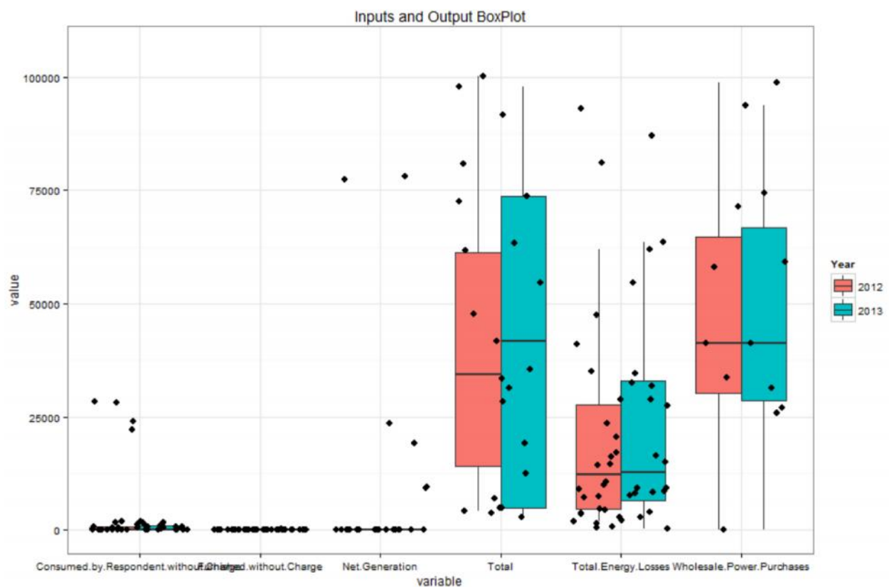
Figure 7 – Box Plot of Inputs and output of efficient DMUs
