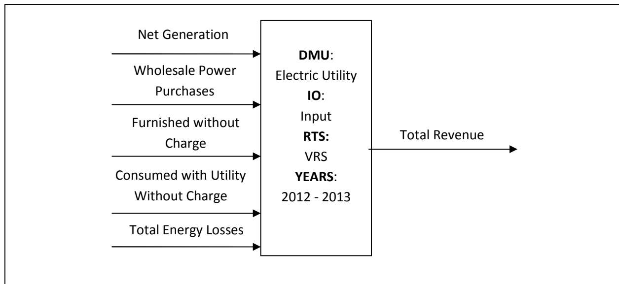
Figure 2: DEA Model
